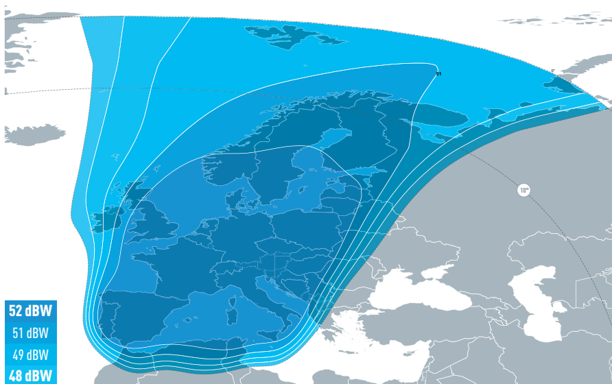
Ku-band Europe Downlink Coverage
