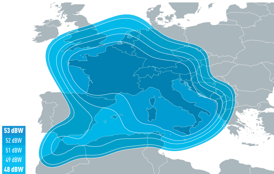
Ku-band Transalpine Downlink Coverage
